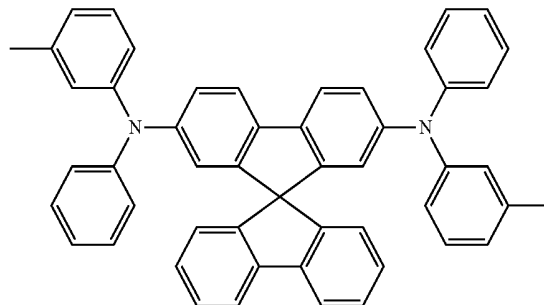
Spiro-NPB
