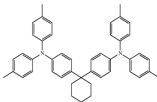
HMTDP
